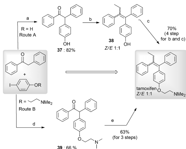
Scheme 1. a) CuI (10 mol %), L8 (10 mol %), Cs 2 CO 3 (4 equiv), tBuOH, 70 °C, 24 h; b) 1. EtMgBr (3 equiv), THF, 25 °C, 5 h, 2. HCl (37%), MeOH, 65 °C, 15 h, 3. tBuOK (4 equiv), DMSO, 50 °C, 2 h; c) NaH (3 equiv), ClC 2 H 4 NMe 2 (2 equiv), DMF, 50 °C, 3 h. d) CuI (10 mol %), L1 (10 mol %), Cs 2 CO 3 (4 equiv), dioxane, 110 °C, 24 h. e) 1. EtMgBr (3 equiv), THF, 25 °C, 5 h, 2. HCl (37%), MeOH, 65 °C, 15 h, 3. tBuOK (5 equiv), DMSO, 50 °C, 2 h.
